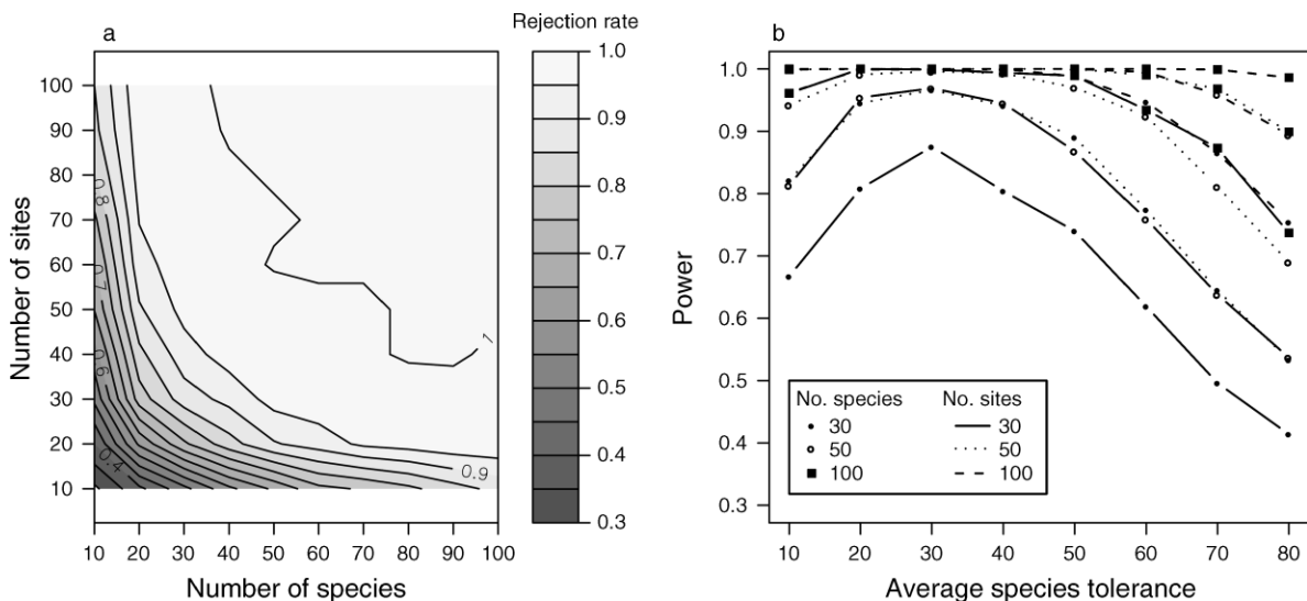
FIG. 4. Results of the power study for the combined approach. The influence on power of (a) the sample size and the number of species and (b) of the species tolerance. The isolines in panel (a) correspond to rejection rates of H_0 (tested against the alternative hypothesis H_3 ) at the 5% significance level after 1000 independent simulations.
