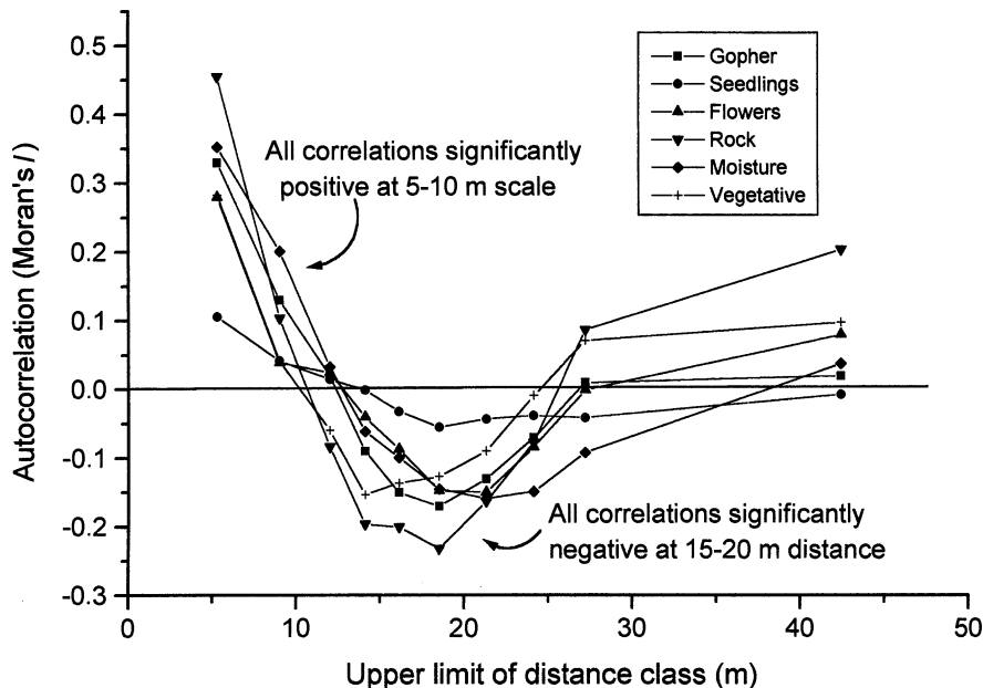
FIG. 3. Correlograms from the Washington Gulch grid of 256 \times 2 \text{ m} quadrats for the six variables described in Methods . Moran's autocorrelation statistic I indicates how similar are values of the variable in quadrats that are separated by the distance class indicated. For all variables, there is significant positive autocorrelation in nearby quadrats and significant negative autocorrelation at distances of 15–20 m, indicating that all the variables are highly patchy and show similar scales of patch structure.
